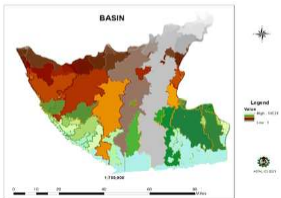
Figure 6: Basin map of Bayelsa State accumulation
