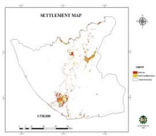
Figure 11: Showing Flooded and non-flooded in 2020
