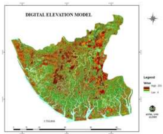
Figure 5: DEM map of Bayelsa State
