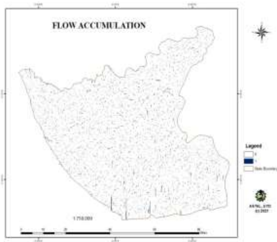
Figure 8: Showing Flow accumulation of 500 meters
